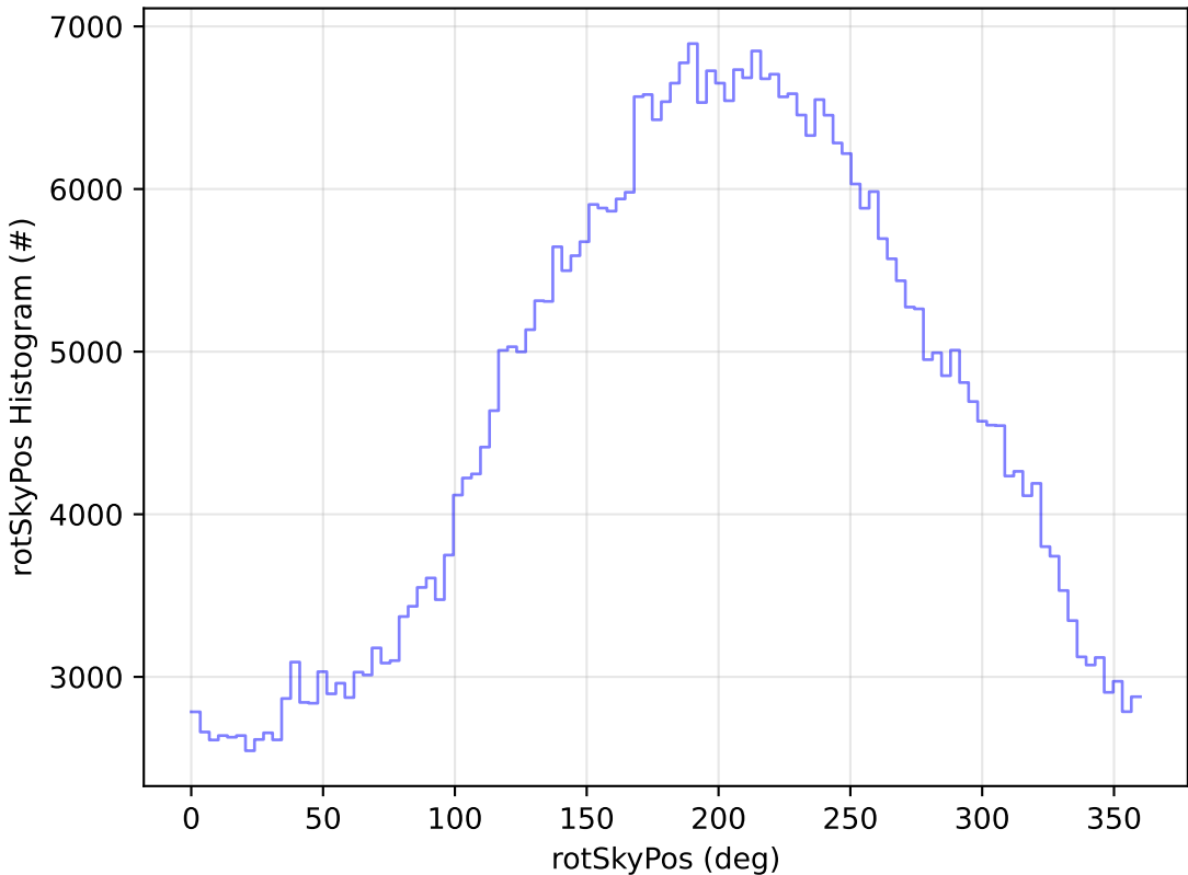
too_elab_r128_d3_gz_v3.4_10yrs All sky r band: rotSkyPos Histogram
