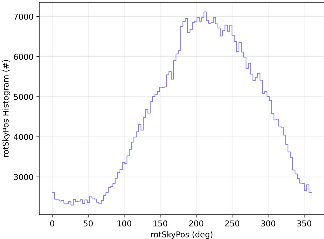
too_elab_r128_d3_gz_v3.4_10yrs All sky i band: rotSkyPos Histogram
