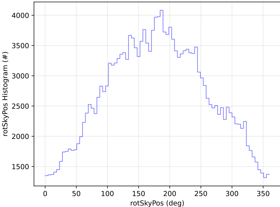
too_elab_r128_d3_gz_v3.4_10yrs All sky g band: rotSkyPos Histogram
