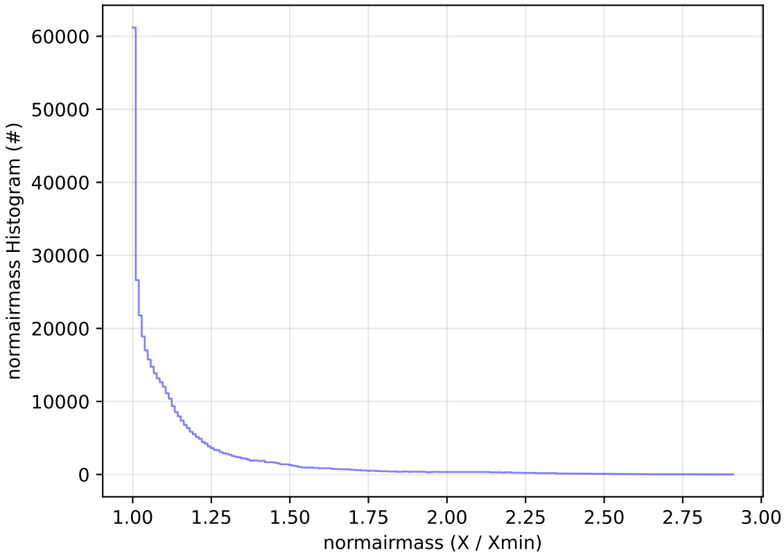
too_elab_r128_d3_gz_v3.4_10yrs WFD z band: normairmass Histogram
