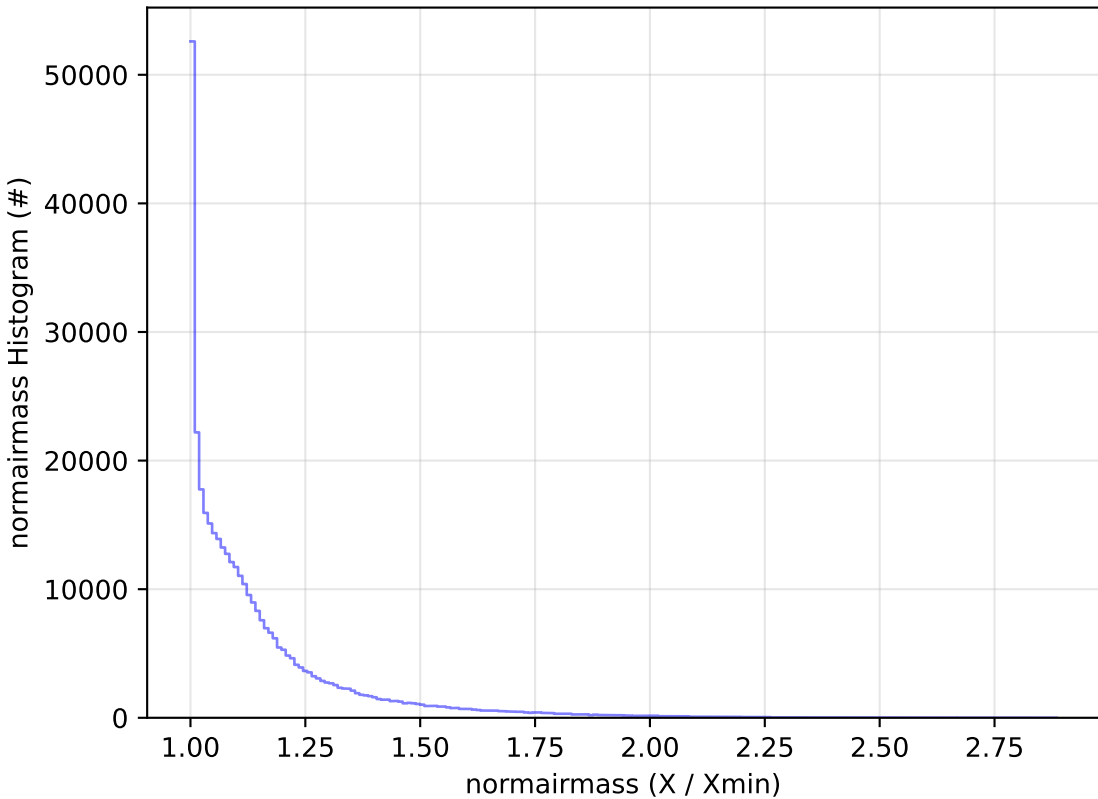
too_elab_r128_d3_gz_v3.4_10yrs WFD y band: normairmass Histogram
