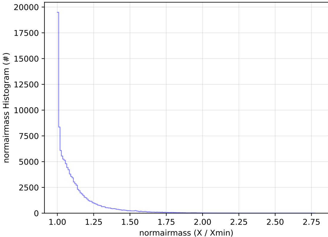
too_elab_r128_d3_gz_v3.4_10yrs WFD u band: normairmass Histogram
