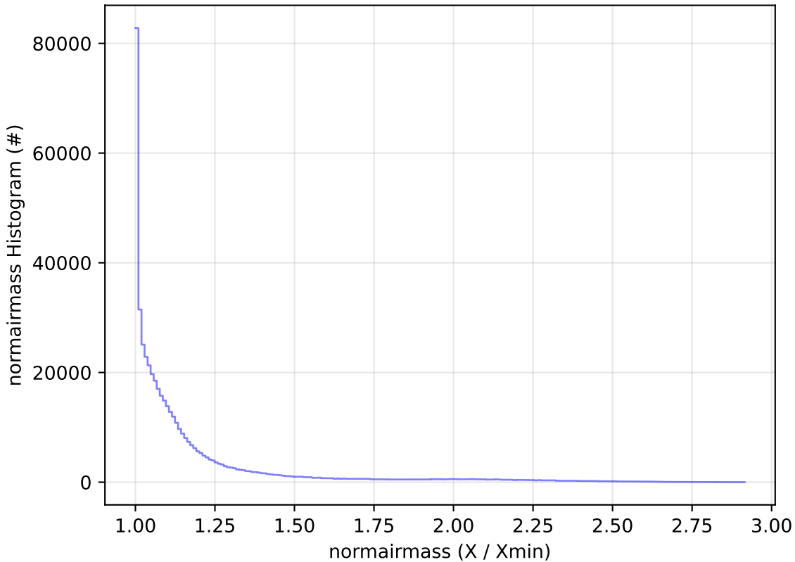
too_elab_r128_d3_gz_v3.4_10yrs WFD i band: normairmass Histogram
