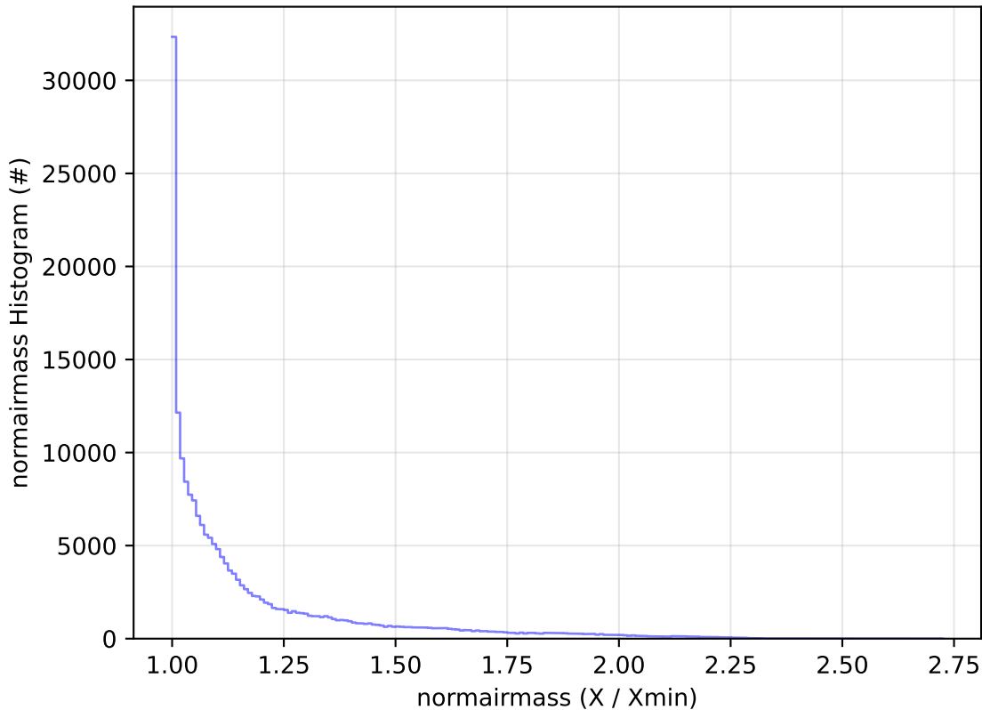
too_elab_r128_d3_gz_v3.4_10yrs WFD g band: normairmass Histogram
