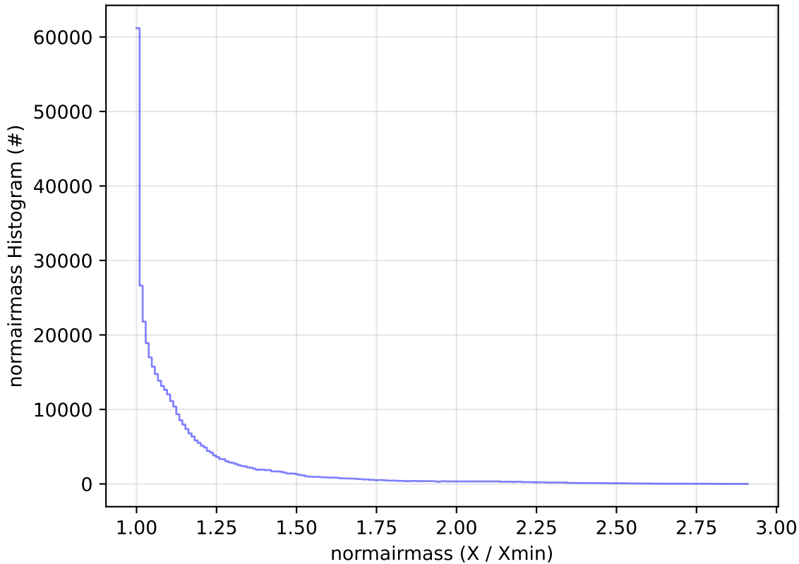
too_elab_r128_d3_gz_v3.4_10yrs All sky z band: normairmass Histogram
