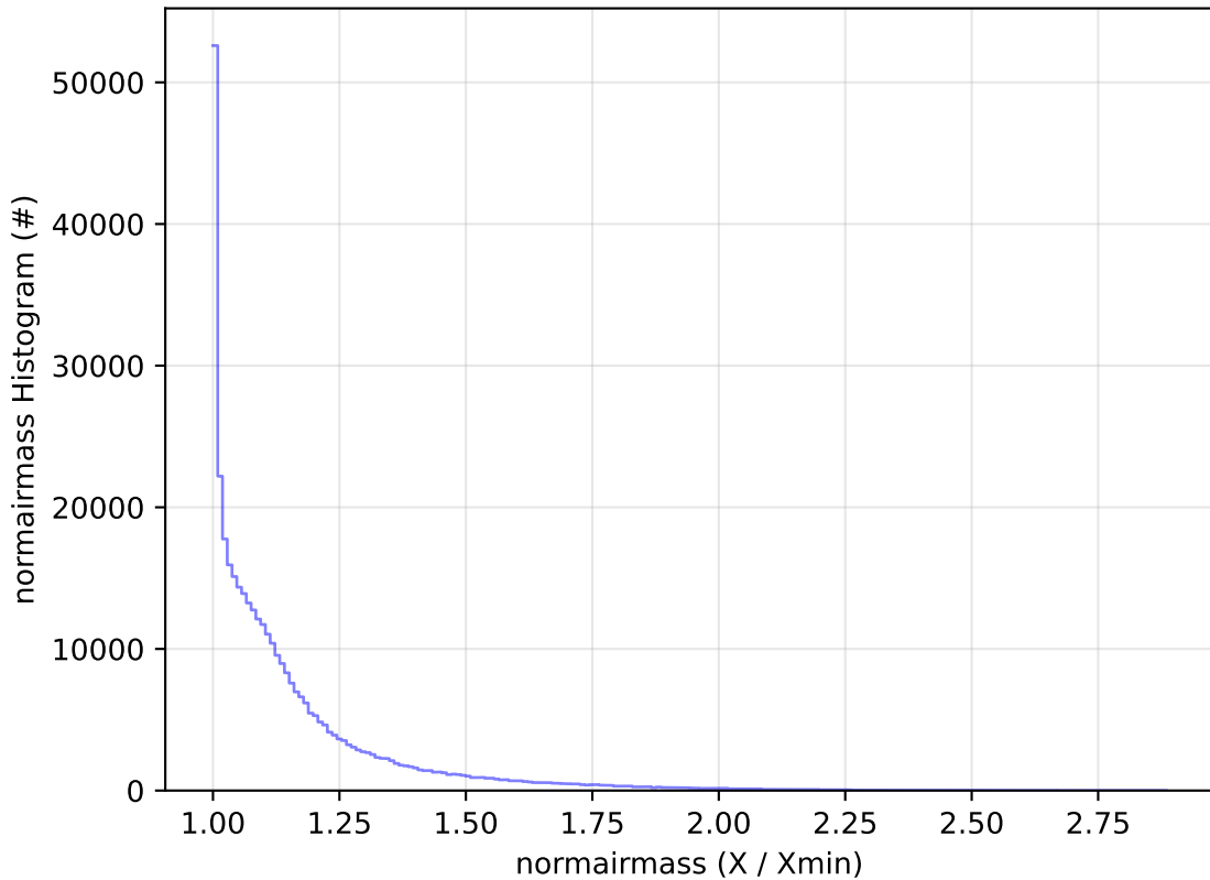
too_elab_r128_d3_gz_v3.4_10yrs All sky y band: normairmass Histogram
