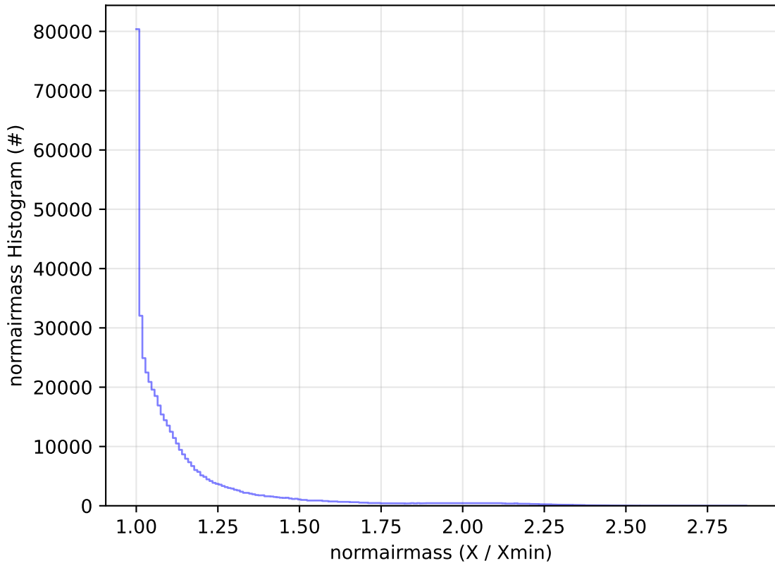
too_elab_r128_d3_gz_v3.4_10yrs All sky r band: normairmass Histogram
