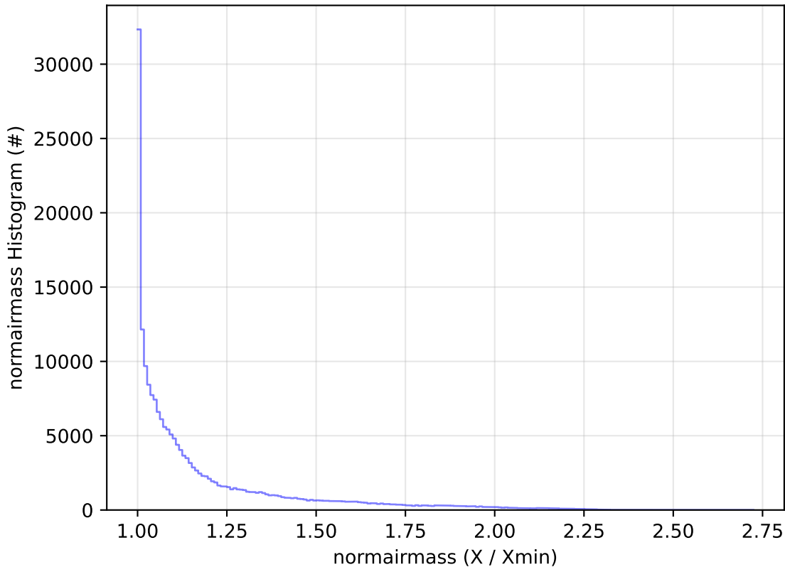
too_elab_r128_d3_gz_v3.4_10yrs All sky g band: normairmass Histogram
