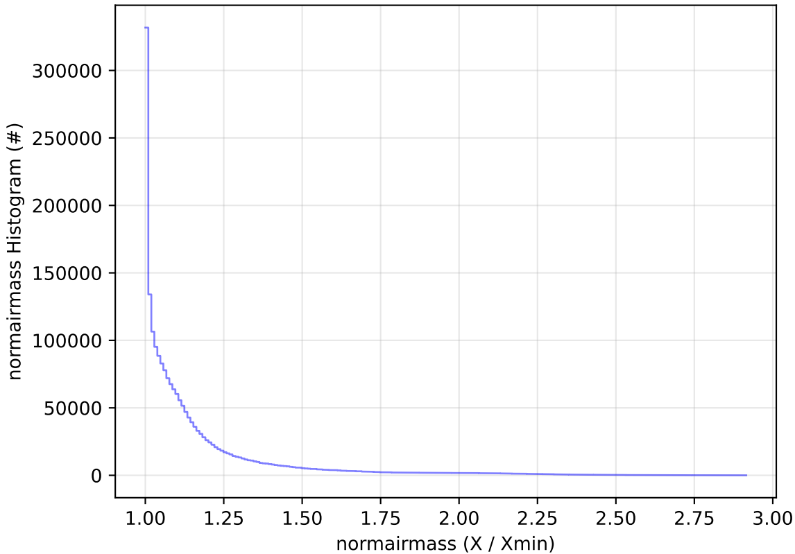
too_elab_r128_d3_gz_v3.4_10yrs All sky all bands: normairmass Histogram
