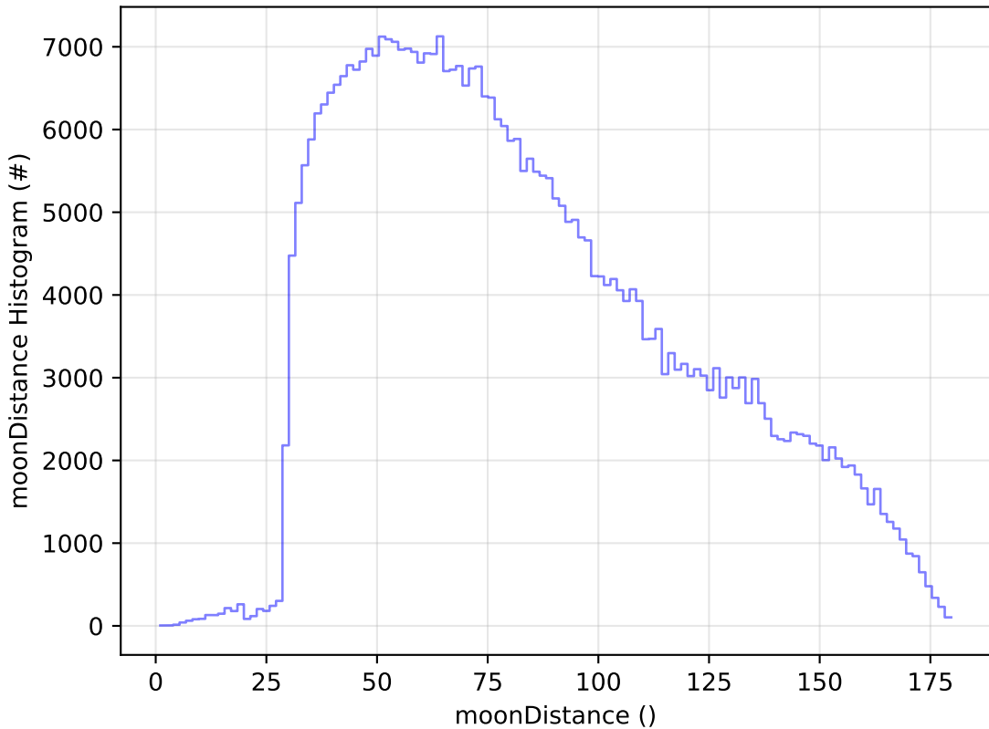
too_elab_r128_d3_gz_v3.4_10yrs WFD z band: moonDistance Histogram
