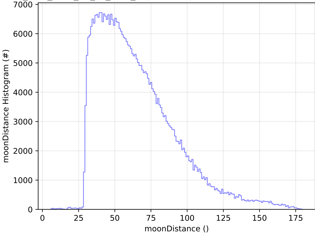
too_elab_r128_d3_gz_v3.4_10yrs WFD y band: moonDistance Histogram
