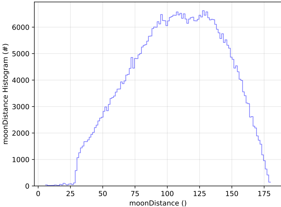
too_elab_r128_d3_gz_v3.4_10yrs WFD r band: moonDistance Histogram
