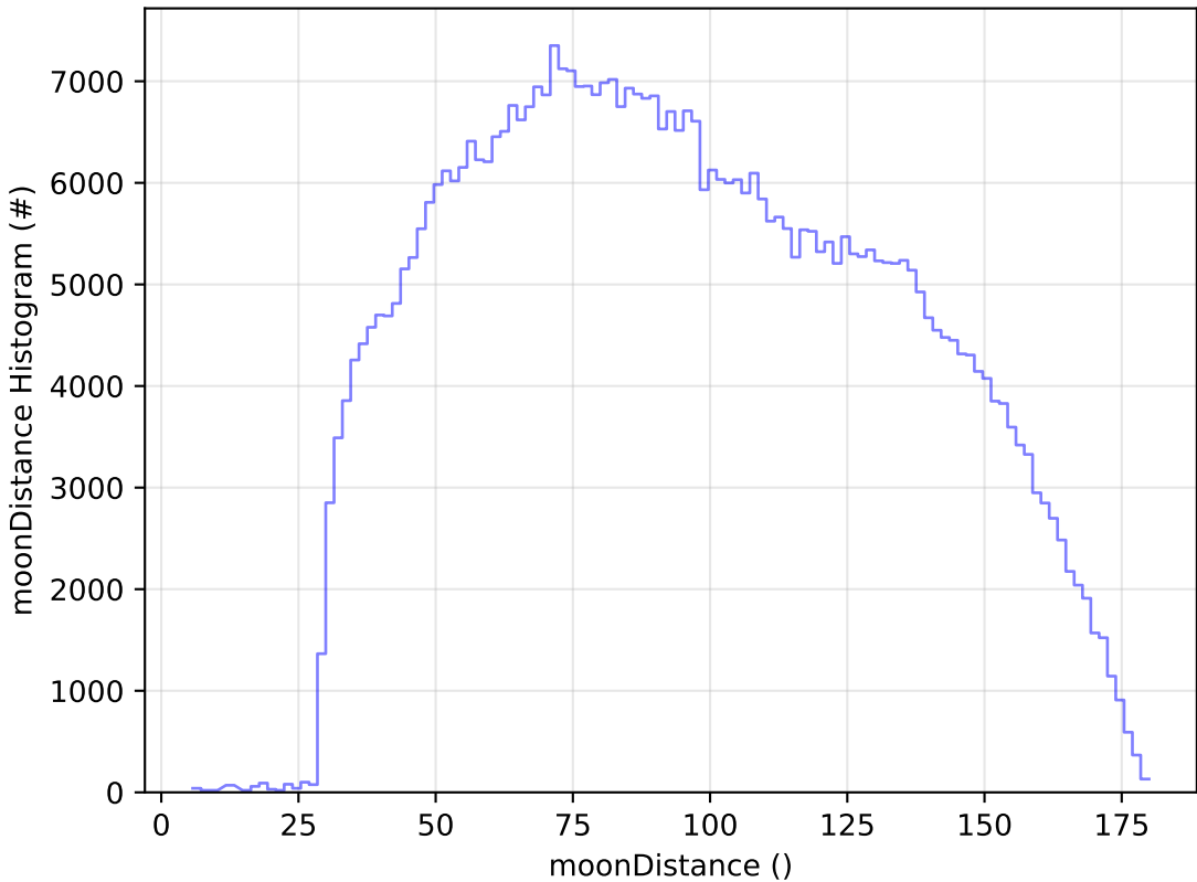
too_elab_r128_d3_gz_v3.4_10yrs WFD i band: moonDistance Histogram
