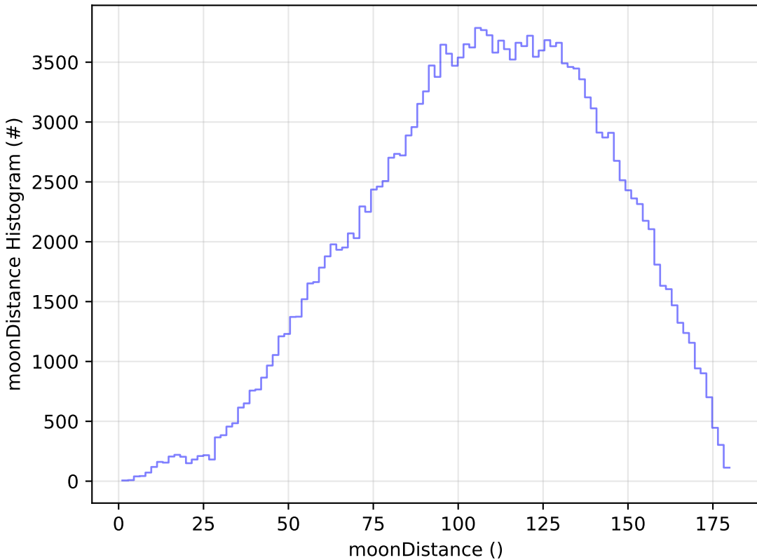
too_elab_r128_d3_gz_v3.4_10yrs WFD g band: moonDistance Histogram
