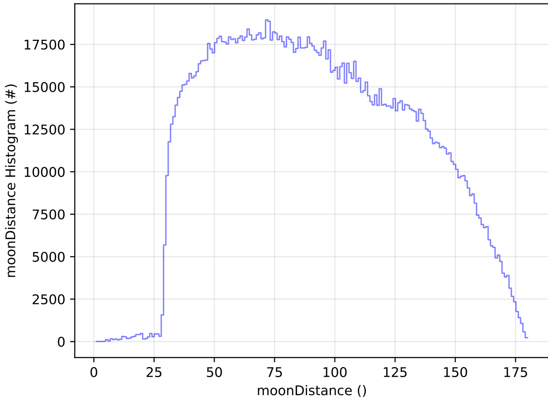
too_elab_r128_d3_gz_v3.4_10yrs WFD all bands: moonDistance Histogram
