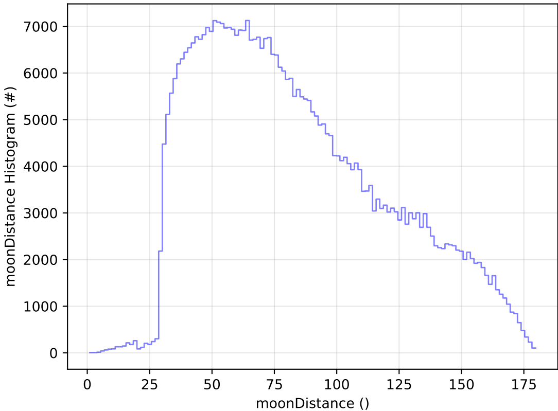
too_elab_r128_d3_gz_v3.4_10yrs All sky z band: moonDistance Histogram
