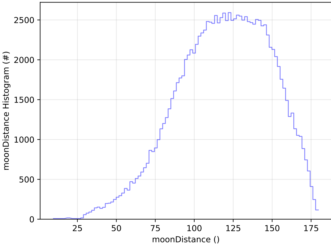
too_elab_r128_d3_gz_v3.4_10yrs All sky u band: moonDistance Histogram
