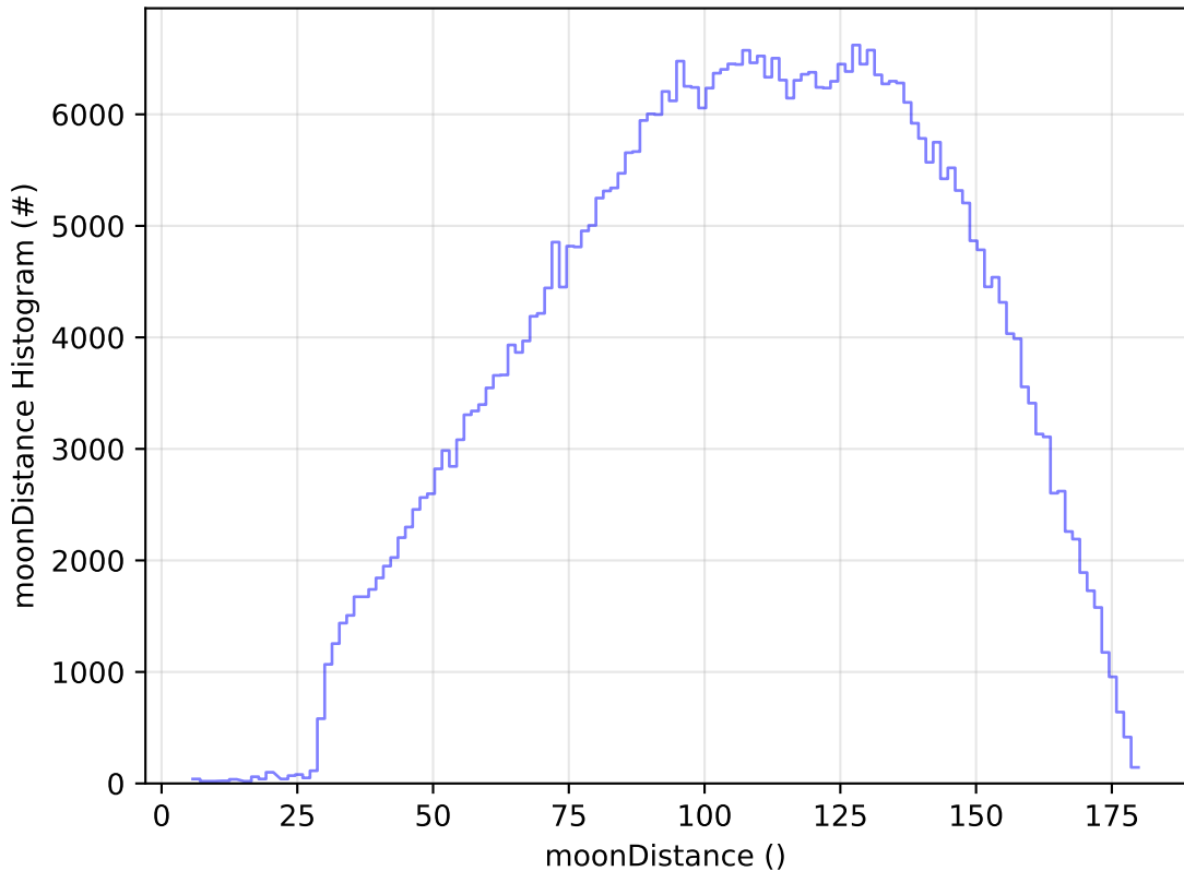
too_elab_r128_d3_gz_v3.4_10yrs All sky r band: moonDistance Histogram
