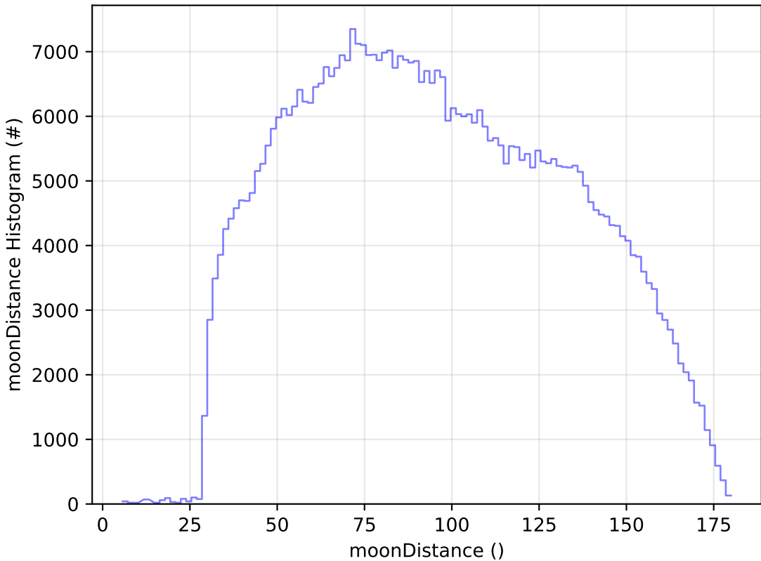
too_elab_r128_d3_gz_v3.4_10yrs All sky i band: moonDistance Histogram
