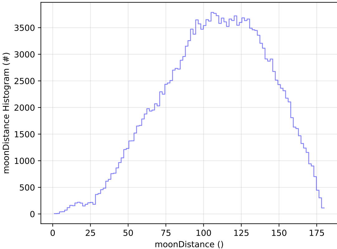
too_elab_r128_d3_gz_v3.4_10yrs All sky g band: moonDistance Histogram
