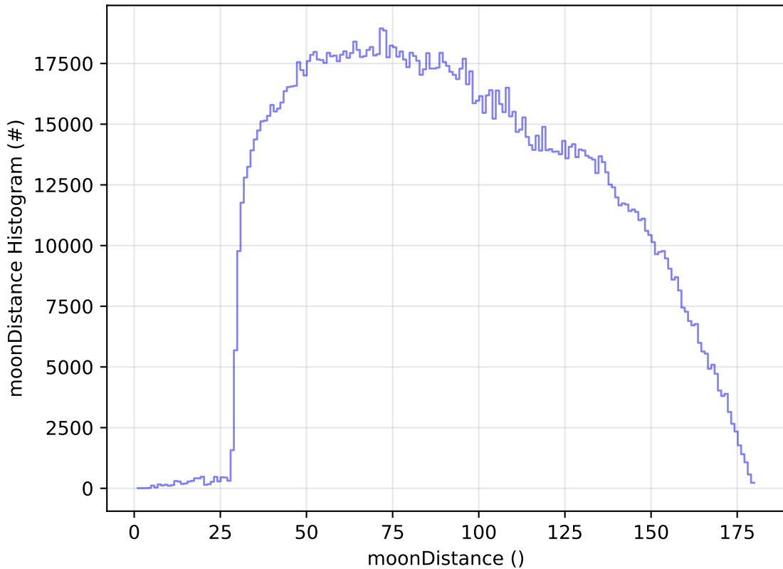
too_elab_r128_d3_gz_v3.4_10yrs All sky all bands: moonDistance Histogram
