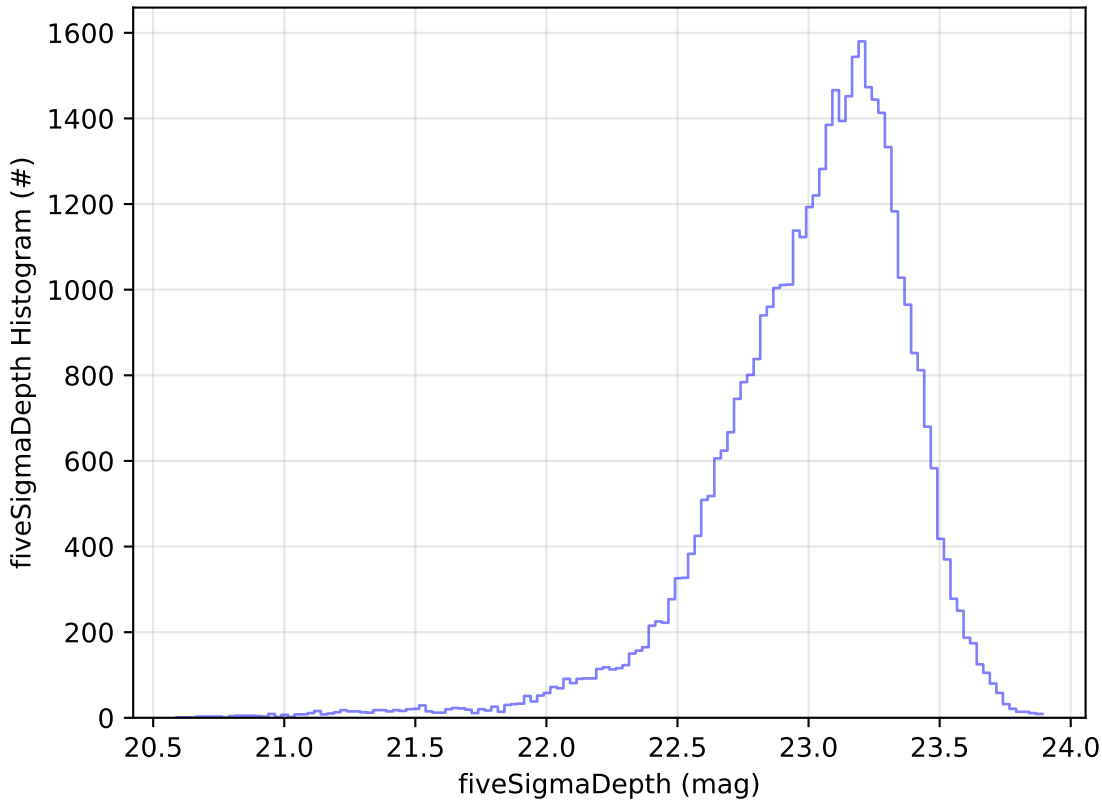
too_elab_r128_d3_gz_v3.4_10yrs Yr 1 z band: fiveSigmaDepth Histogram
