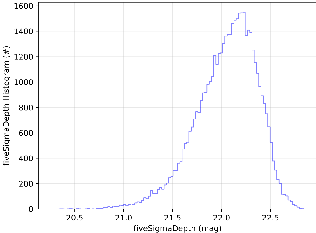
too_elab_r128_d3_gz_v3.4_10yrs Yr 1 y band: fiveSigmaDepth Histogram
