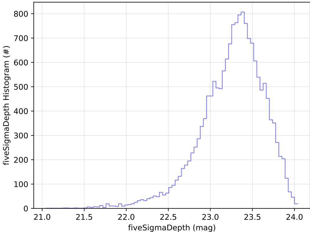
too_elab_r128_d3_gz_v3.4_10yrs Yr 1 u band: fiveSigmaDepth Histogram
