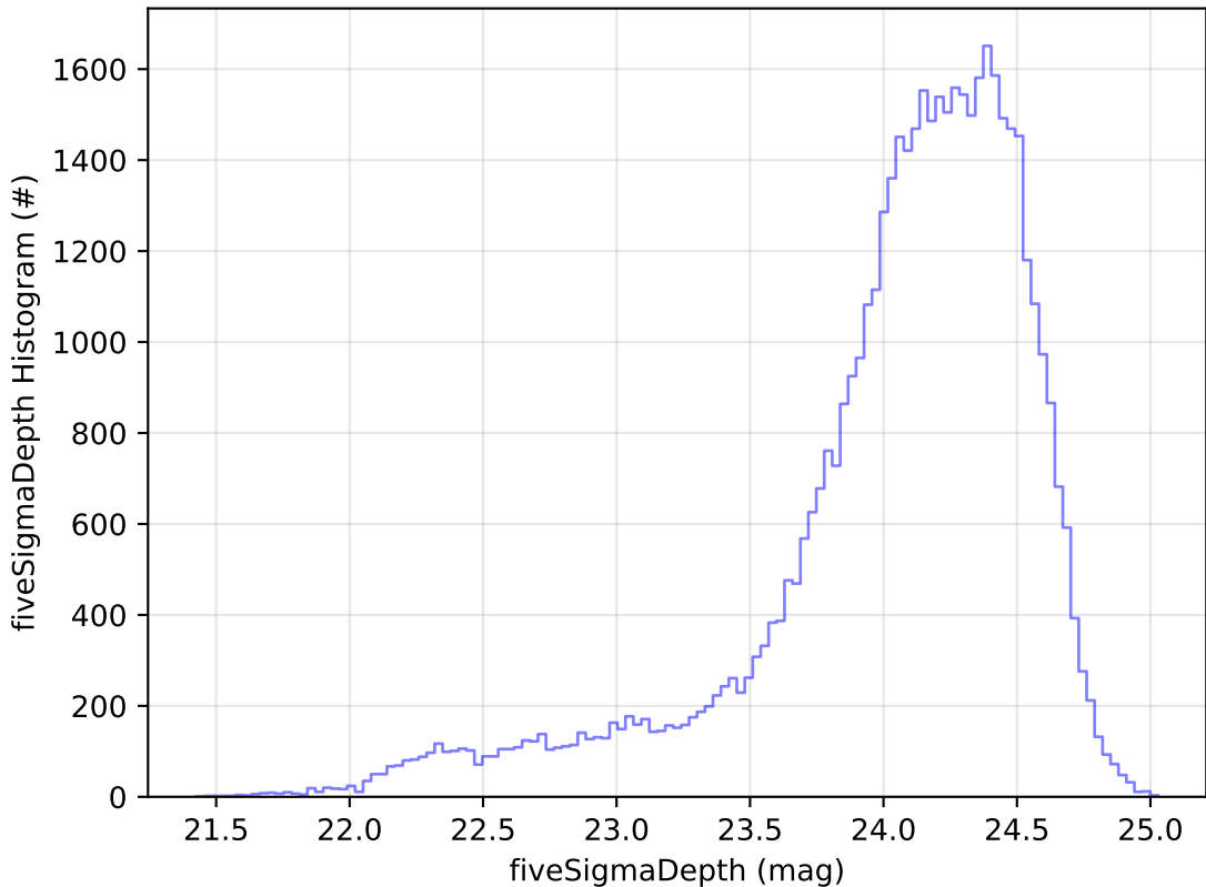
too_elab_r128_d3_gz_v3.4_10yrs Yr 1 r band: fiveSigmaDepth Histogram
