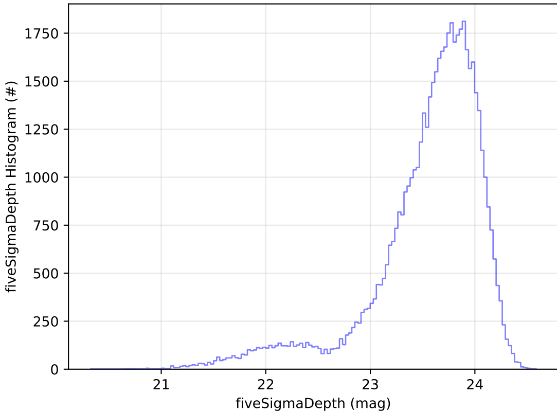
too_elab_r128_d3_gz_v3.4_10yrs Yr 1 i band: fiveSigmaDepth Histogram
