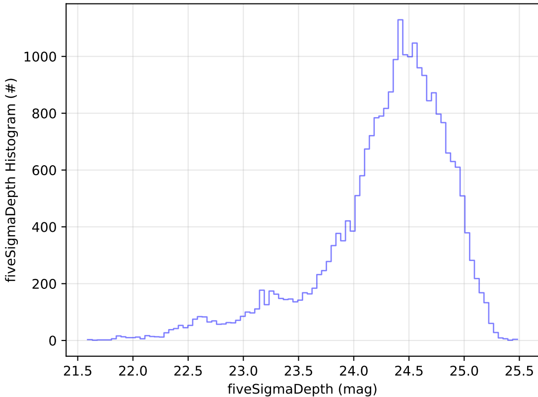
too_elab_r128_d3_gz_v3.4_10yrs Yr 1 g band: fiveSigmaDepth Histogram
