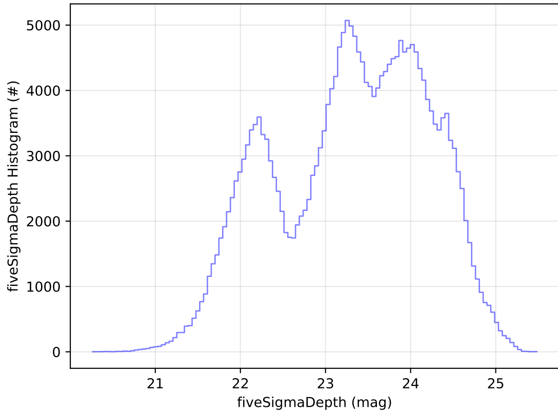
too_elab_r128_d3_gz_v3.4_10yrs Yr 1 all bands: fiveSigmaDepth Histogram
