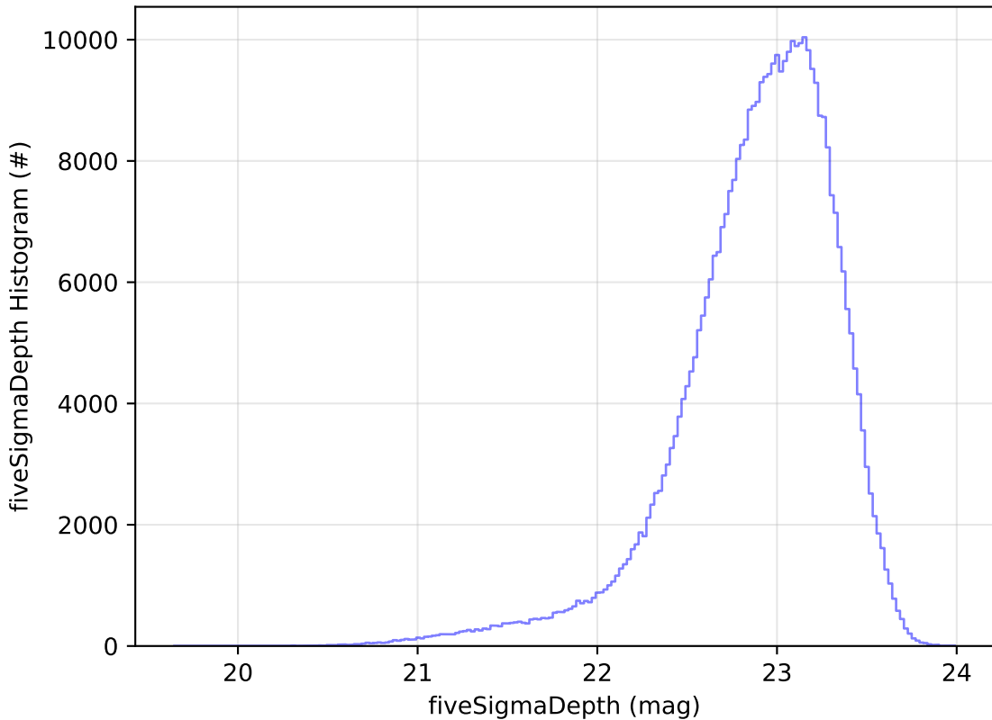
too_elab_r128_d3_gz_v3.4_10yrs WFD z band: fiveSigmaDepth Histogram
