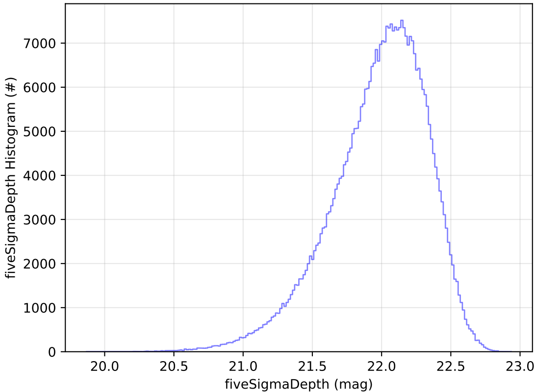
too_elab_r128_d3_gz_v3.4_10yrs WFD y band: fiveSigmaDepth Histogram
