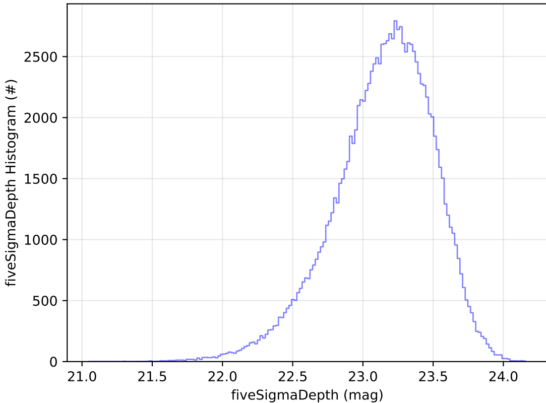
too_elab_r128_d3_gz_v3.4_10yrs WFD u band: fiveSigmaDepth Histogram
