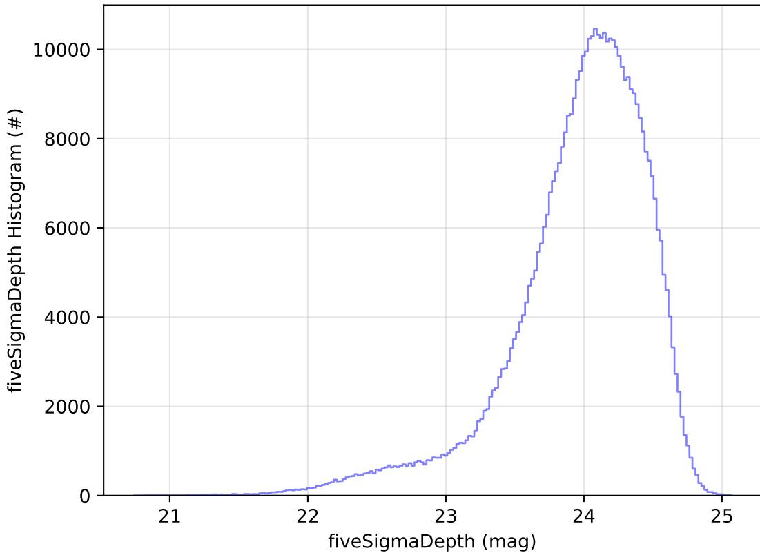
too_elab_r128_d3_gz_v3.4_10yrs WFD r band: fiveSigmaDepth Histogram
