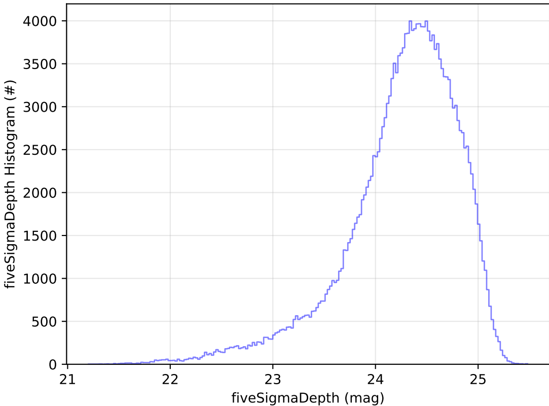
too_elab_r128_d3_gz_v3.4_10yrs WFD g band: fiveSigmaDepth Histogram
