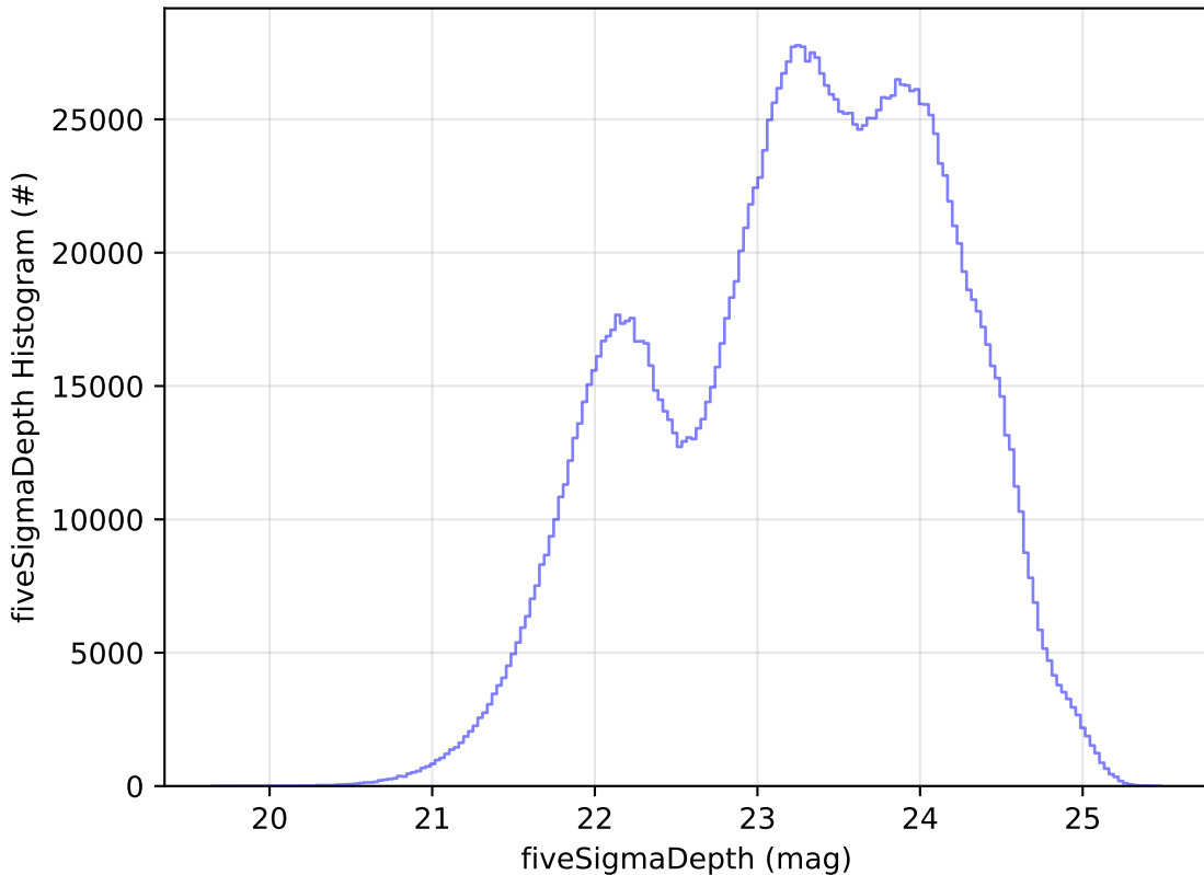
too_elab_r128_d3_gz_v3.4_10yrs WFD all bands: fiveSigmaDepth Histogram
