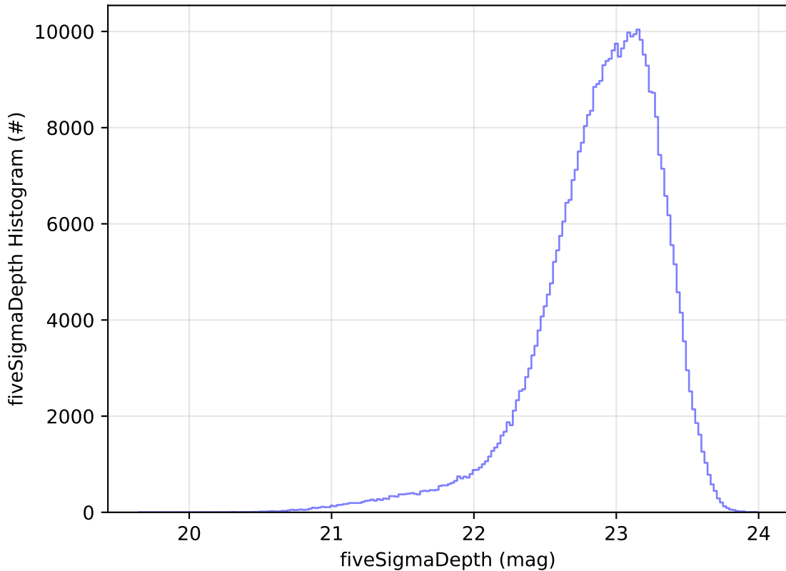
too_elab_r128_d3_gz_v3.4_10yrs All sky z band: fiveSigmaDepth Histogram
