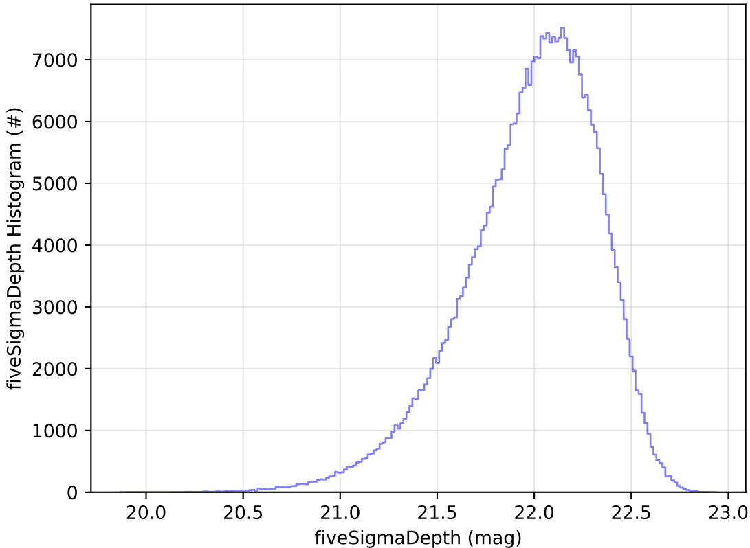
too_elab_r128_d3_gz_v3.4_10yrs All sky y band: fiveSigmaDepth Histogram
