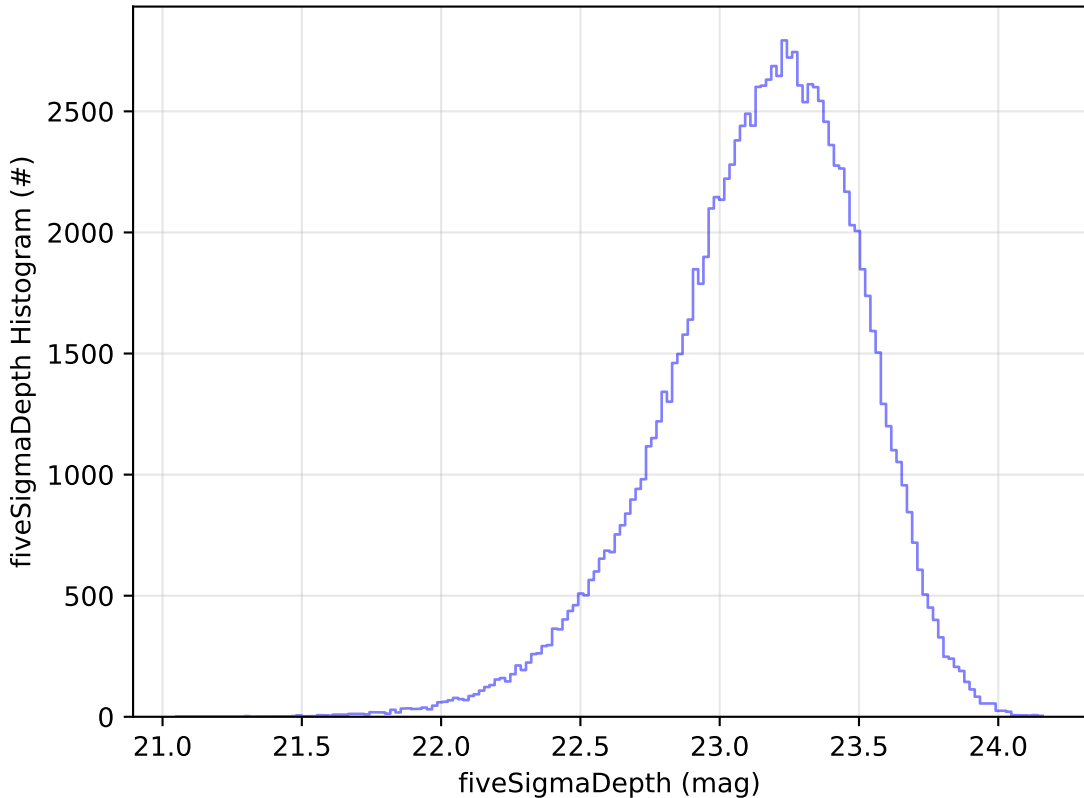
too_elab_r128_d3_gz_v3.4_10yrs All sky u band: fiveSigmaDepth Histogram
