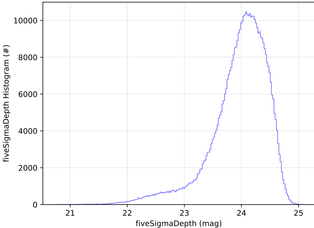
too_elab_r128_d3_gz_v3.4_10yrs All sky r band: fiveSigmaDepth Histogram
