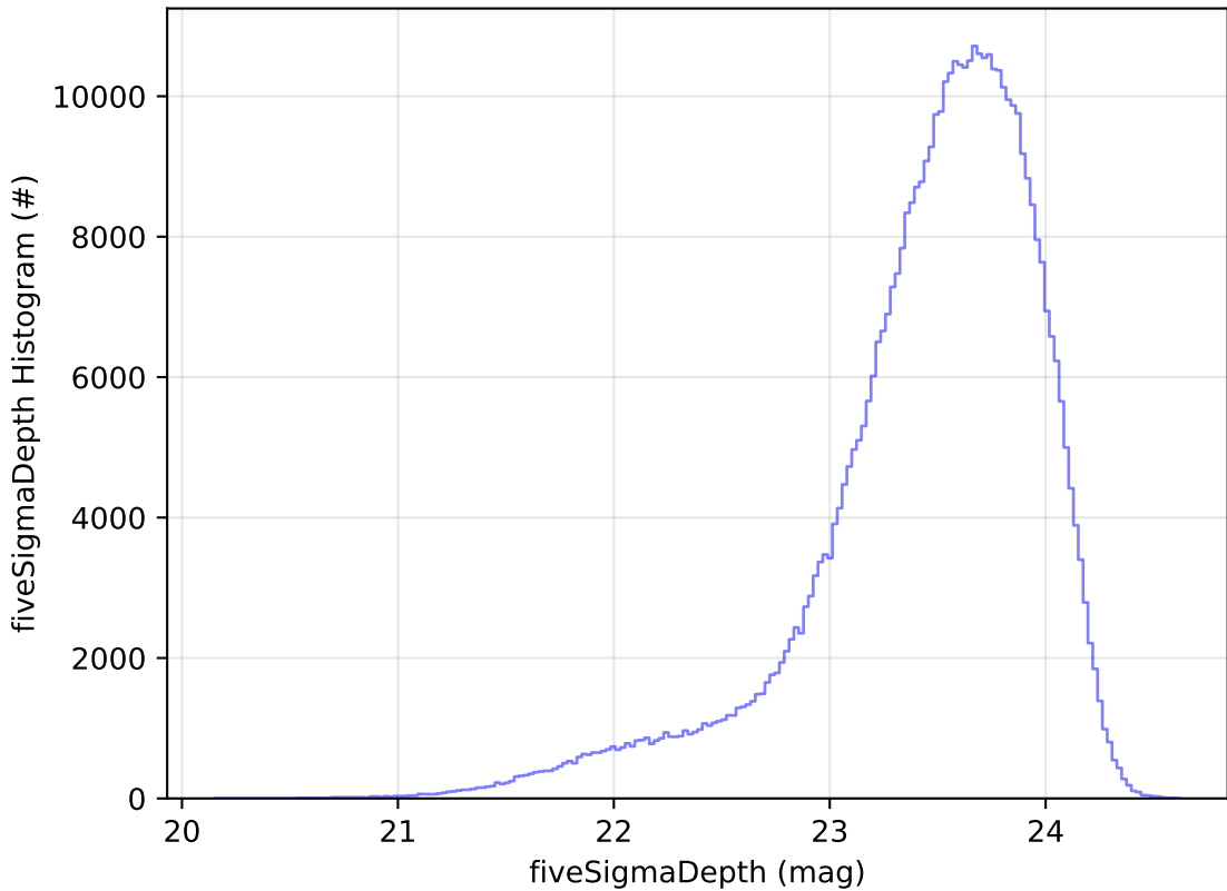
too_elab_r128_d3_gz_v3.4_10yrs All sky i band: fiveSigmaDepth Histogram
