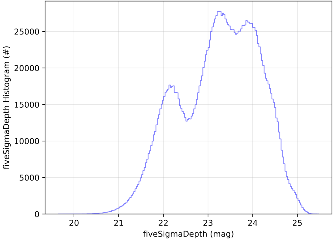
too_elab_r128_d3_gz_v3.4_10yrs All sky all bands: fiveSigmaDepth Histogram
