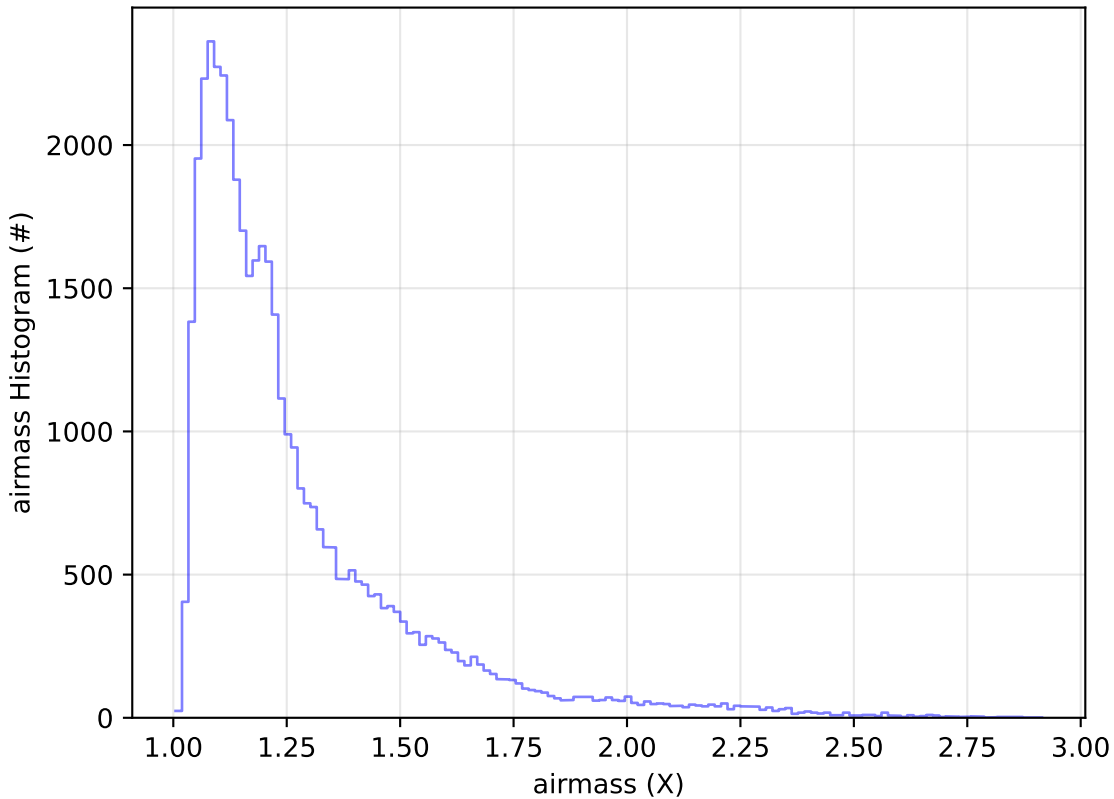
too_elab_r128_d3_gz_v3.4_10yrs Yr 1 z band: airmass Histogram
