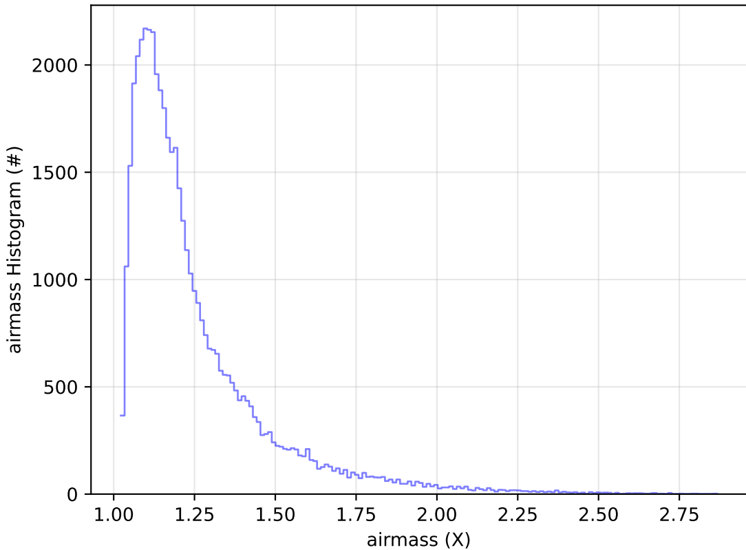
too_elab_r128_d3_gz_v3.4_10yrs Yr 1 y band: airmass Histogram
