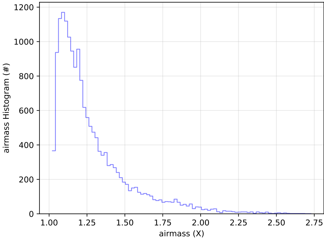
too_elab_r128_d3_gz_v3.4_10yrs Yr 1 u band: airmass Histogram
