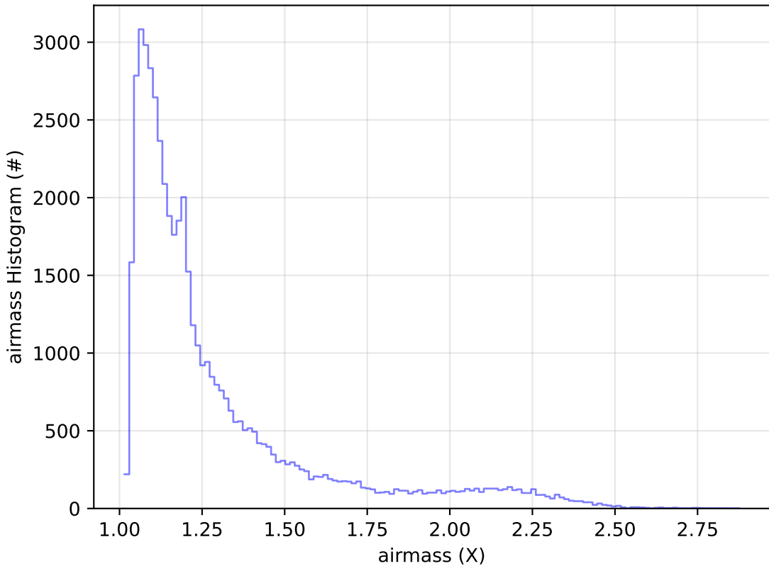
too_elab_r128_d3_gz_v3.4_10yrs Yr 1 r band: airmass Histogram
