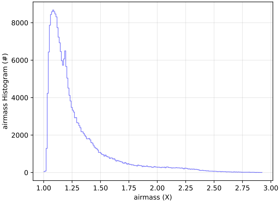
too_elab_r128_d3_gz_v3.4_10yrs Yr 1 all bands: airmass Histogram
