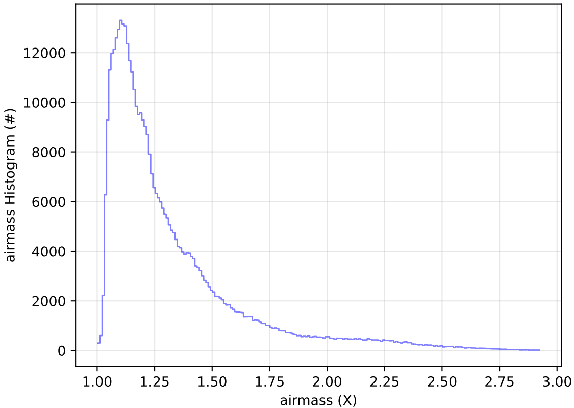
too_elab_r128_d3_gz_v3.4_10yrs WFD z band: airmass Histogram
